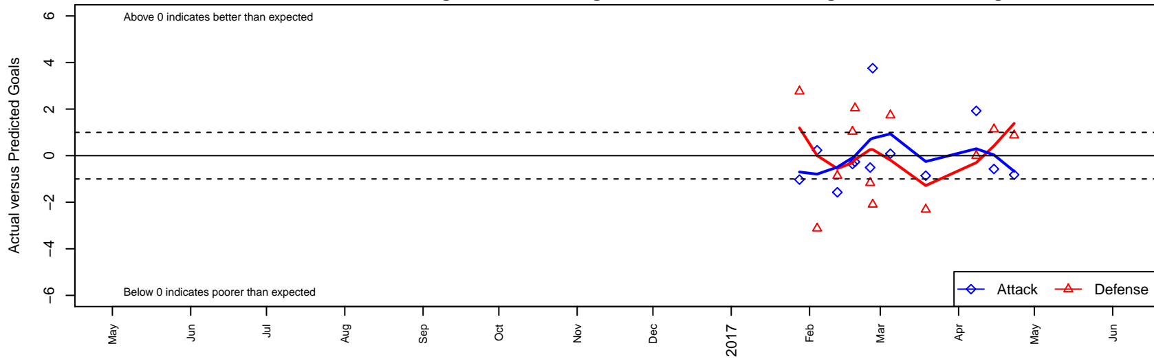
TFA Willamette Gold B00 Dots are actual minus expected GF (blue circles) and GA (red triangles). Blue line is smoothed change in attack strength. Red is smoothed change in defense strength.
